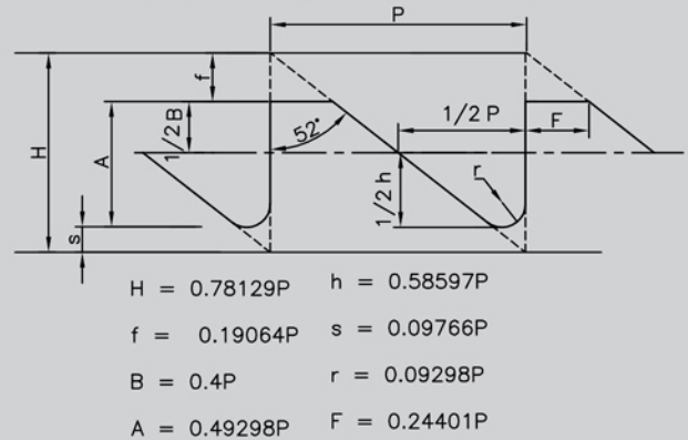
BUTTRESS 0/52° THREAD PROFILE
