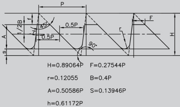
BUTTRESS 7/45° THREAD PROFILE
